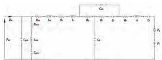
Fig. 1. The model of human respiratory system modeled in the application [15]:
