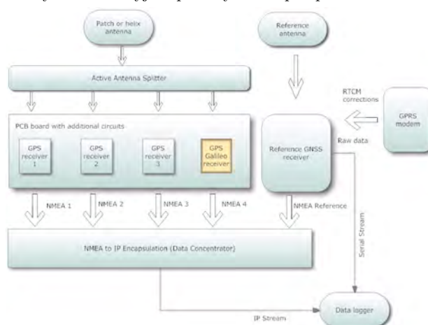
Fig. 4. Structure of connectivity between individual elements of the evaluation board
