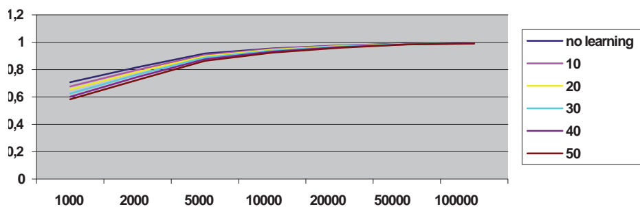
Fig. 1. The plots illustrate the effect of decelerating the rate of evolution for different numbers of the individuals that underwent the process of learning (mutation intensity was set at 10 % of the population)
