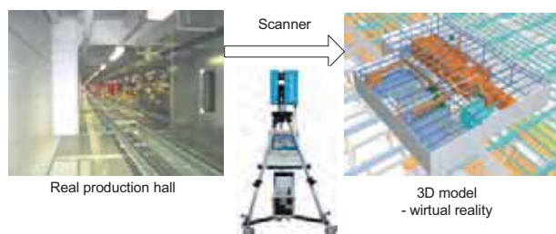
Fig. 2. Digitizing of the manufacturing system
