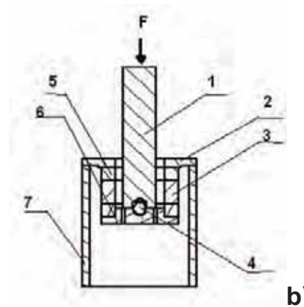
Fig. 7. Method of application of uniform tensile stresses to the ring-shaped sample: a) idea of the method, b) device for practical realization of this idea: 1 – main shaft, 2 – upper backing, 3 – ring-shaped core under investigation, 4 – steel ball, 5 – core backings, 6 – lower backing, 7 – tube
