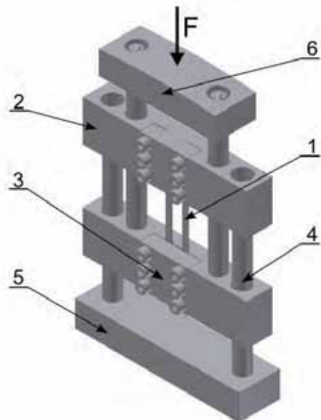
Fig. 4. Mechanical force F reversing system for application of the tensile stresses to the frame-shaped core: 1 – frame-shaped core, 2 – moving element, 3 – sample holder, 4 – column, 5 – base, 6 – upper cover
