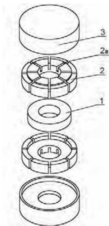
Fig. 6. Schematic diagram of the device for applying the uniform compressive stress to the ring core [12]: 1 – investigated ring core, 2 – nonmagnetic cylindrical backing, 2a – grooves for windings, 3 – base backings
