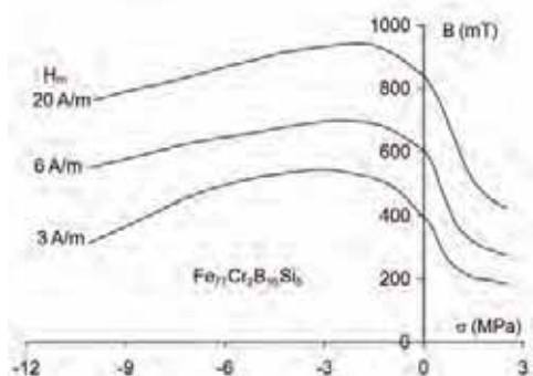
Fig. 8. Magnetoelastic B(\sigma)_H characteristics of amorphous alloy in as-quenched state for constant values of amplitude of magnetizing field H_m
