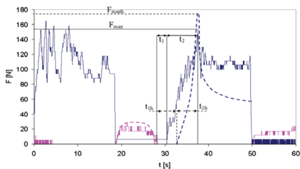
Fig. 8. Real and hypothetical characteristics of maximum braking force, reaction and braking time for the rested and tired driver
