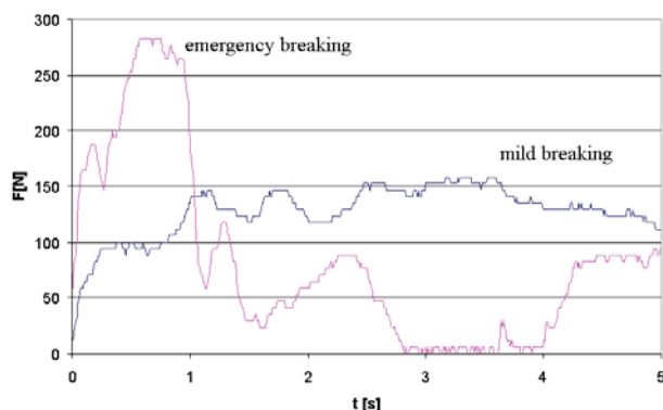
Fig. 7. Measurement of pressure force made during mild and emergency braking while driving in the depot
