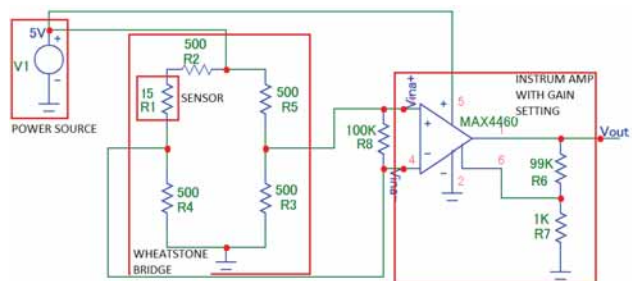
Fig. 11. Measurement system with applied modification
