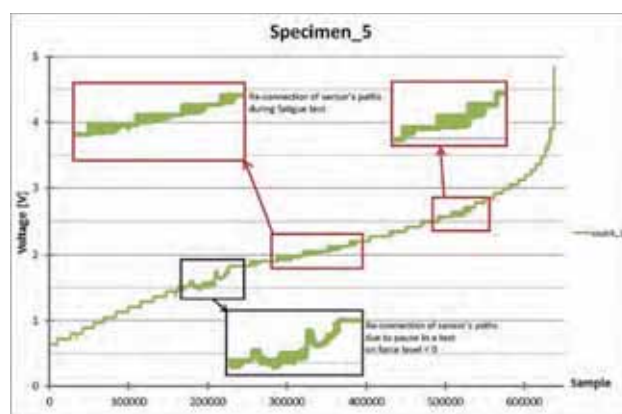
Fig. 9. Measurement data from ladder sensor, specimen 5
