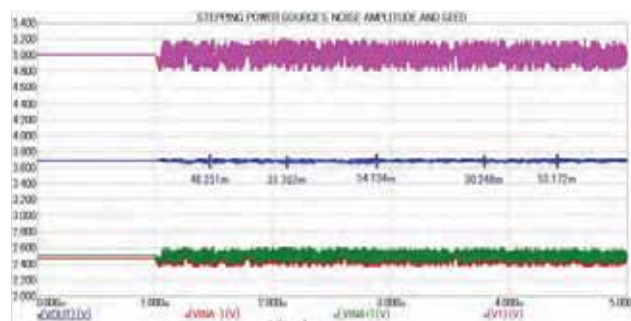
Fig. 13. Influence of power source's amplitude fluctuation on the output signal
