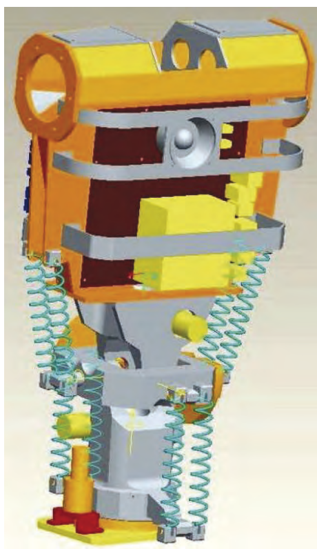
Fig. 3. Engineering drawing of the upper body of the humanoid robot with integrated mainboards, loudspeaker and the 3DOF hip with supporting springs
